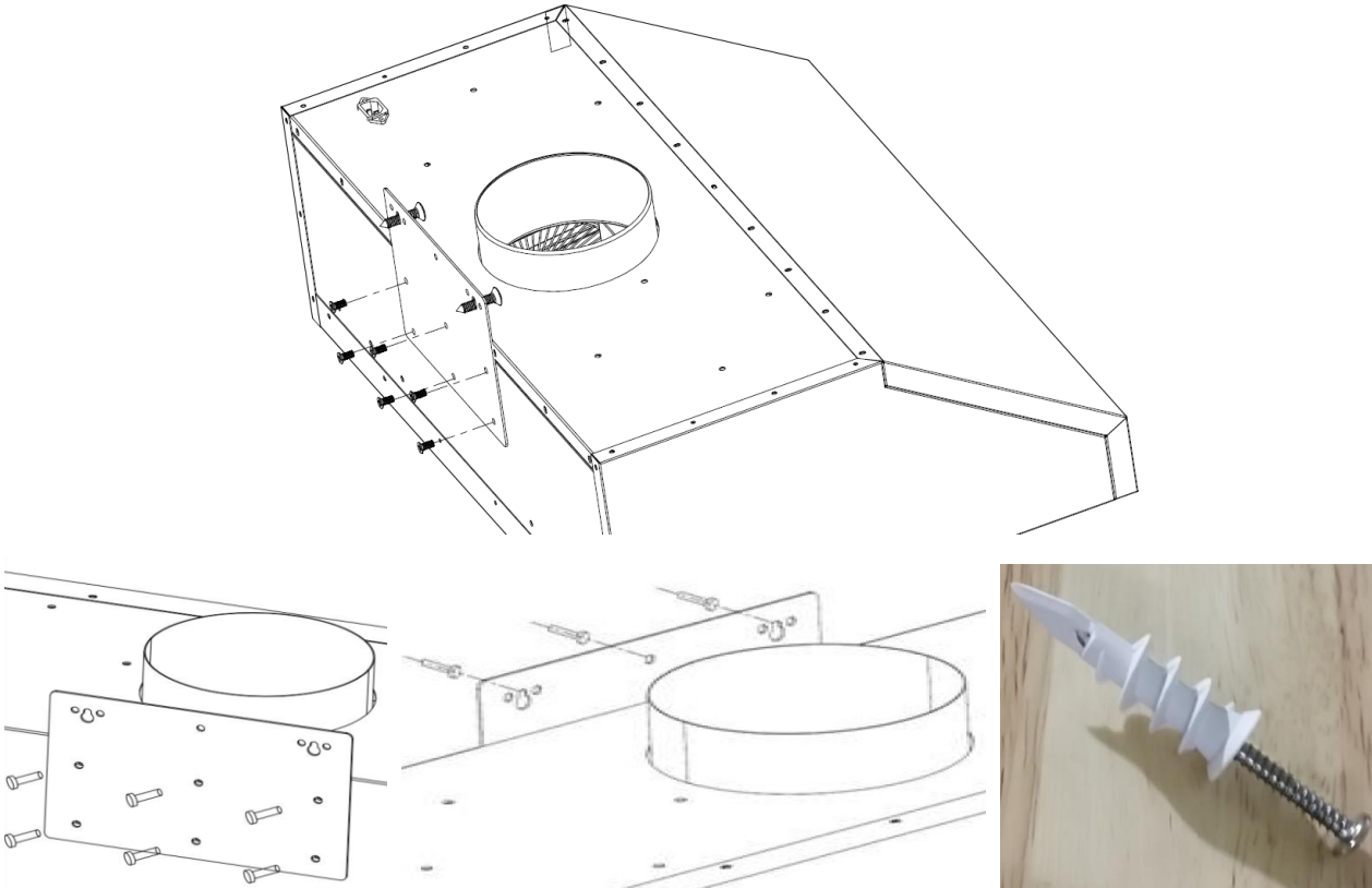
(1) Short Screw Set Mounting
