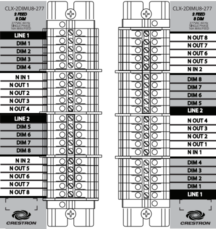
CLT-2DIMU8-277 Terminal Block with Left- and Right-Side CLX-2DIMU8-277 Labels
