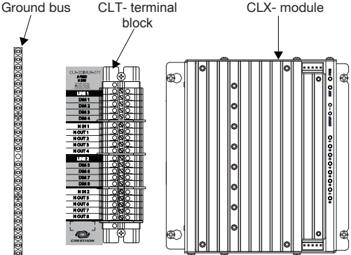
Terminal Block and Module Layout for a Double-Wide Enclosure (CLT-2DIMU8-277 and CLX-2DIMU8-277 Shown)
