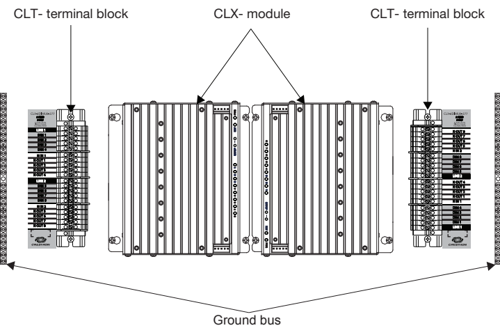
Terminal Block and Module Layout for a Double-Wide Enclosure (CLT-2DIMU8-277 and CLX-2DIMU8-277 Shown)
