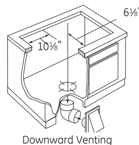
Downward Venting
