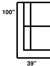
1294-LR/CNR/LL
