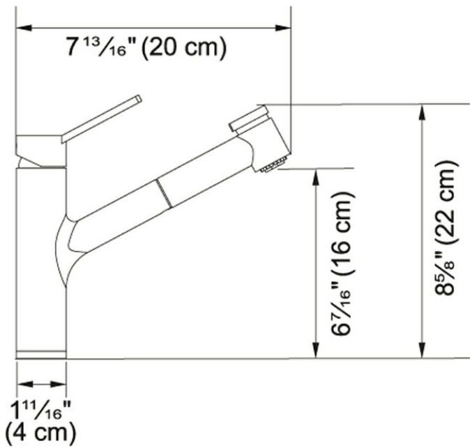
Technical Drawing
