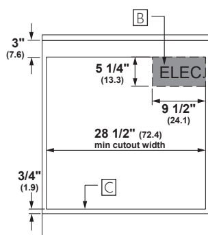
STANDARD INSTALLATION FRONT VIEW
