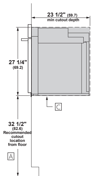
STANDARD INSTALLATION
