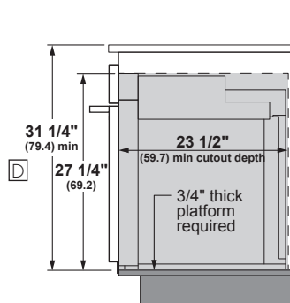
STANDARD INSTALLATION
