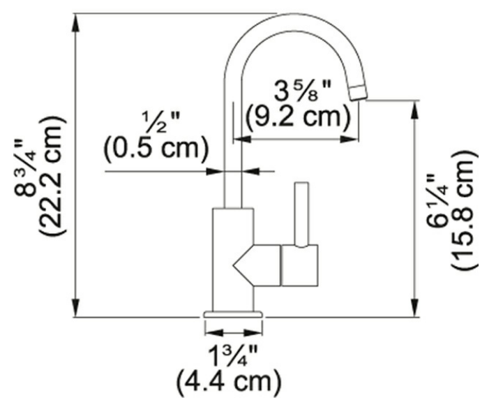
Technical Drawing
