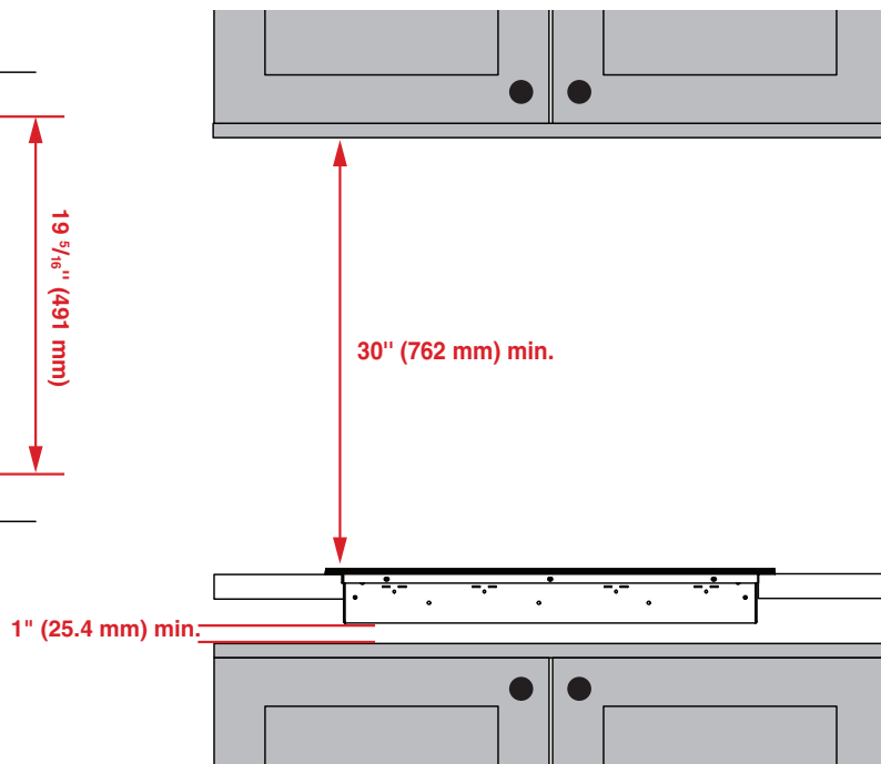
Cabinet Space
