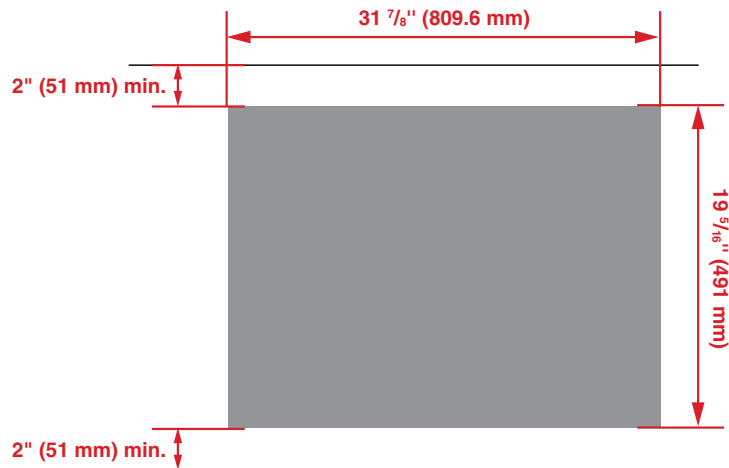
Countertop Cutout
