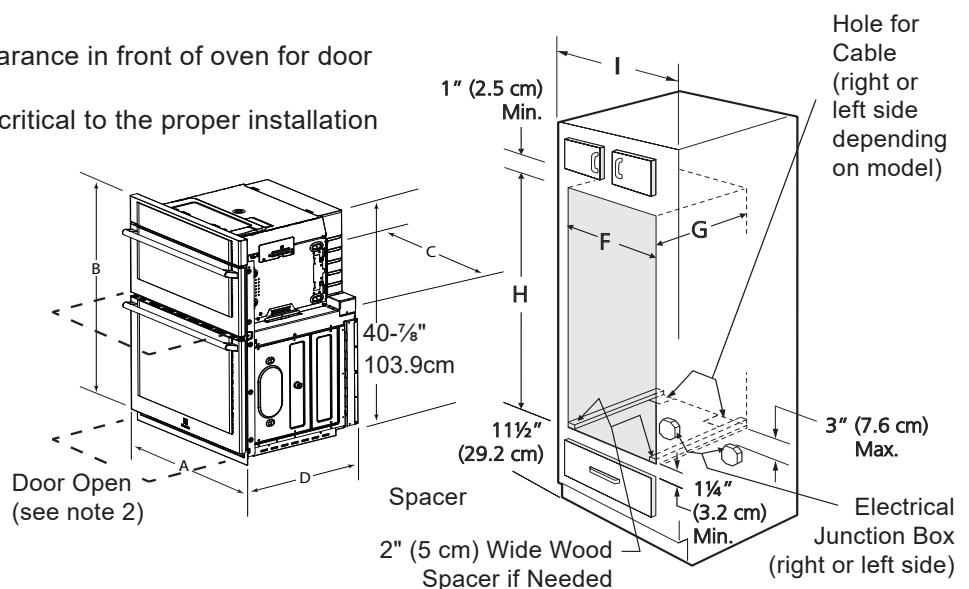
Figure 1: Product and Cutout Dimensions
