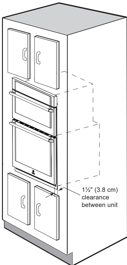
Figure 6: Cabinet Installation
