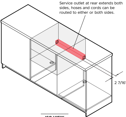
ISO VIEW
