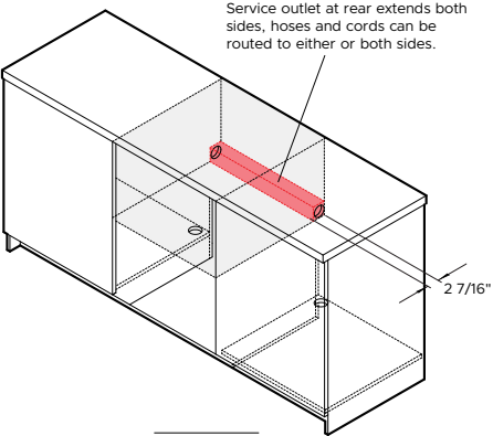
ISO VIEW
