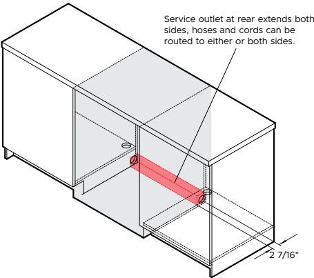
ISO VIEW
