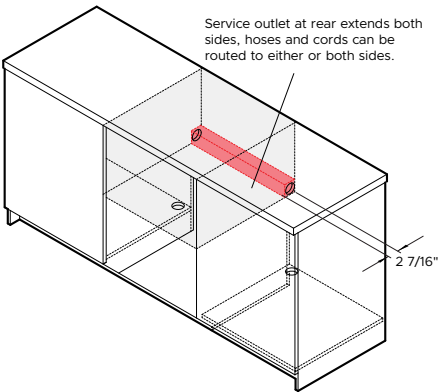
ISO VIEW
