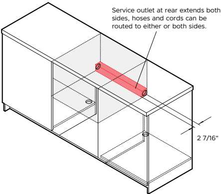
ISO VIEW
