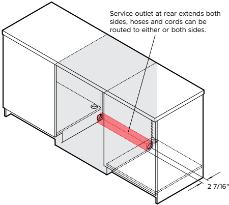
ISO VIEW
