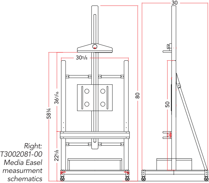
Right and below: T3002081-00 Media Easel W31 D30 H80 One removeable shelf for components, mounting brackets for flat screen TV (hardware not included), castered Opening: W23 H4 Holds up to a 50" flat screen TV Holds up to 99 lbs, adjustable height One fixed shelf, shelf size: W24½ D16 H5
