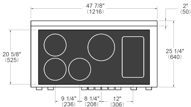
WORKTOP DETAILS
