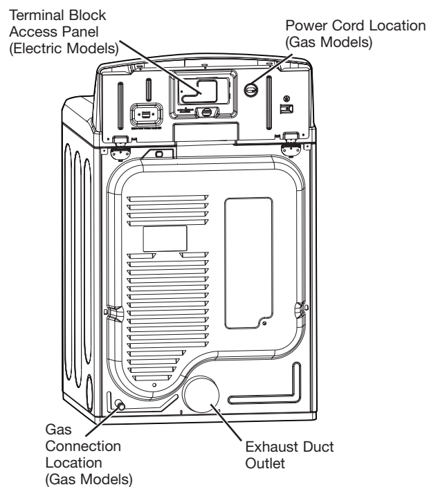
Rear of Dryer
