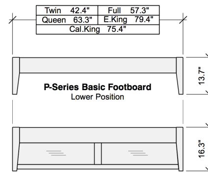
P-Series Basic Footboard Lower Position K-Series Basic Footboard Upper Position
