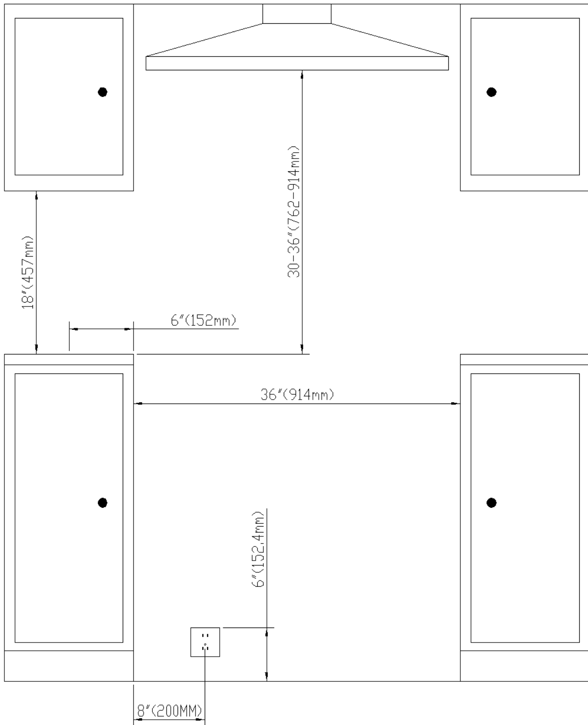
Front View
