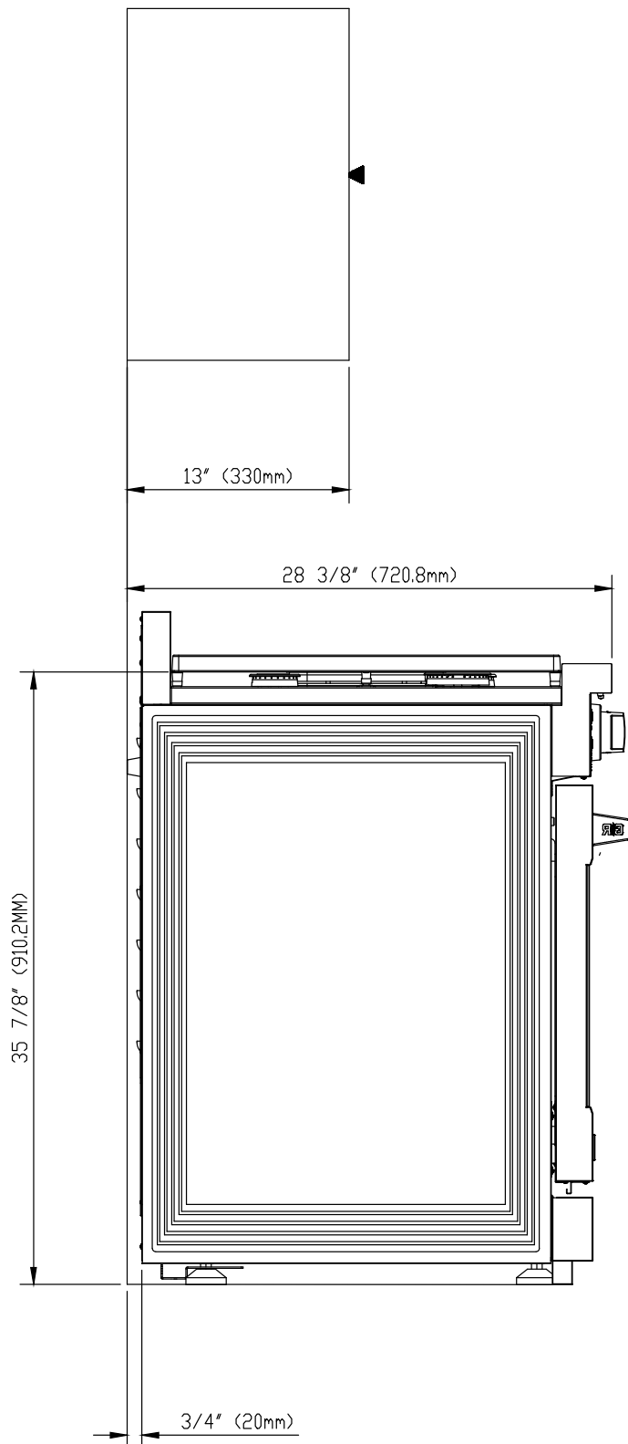
Side View
