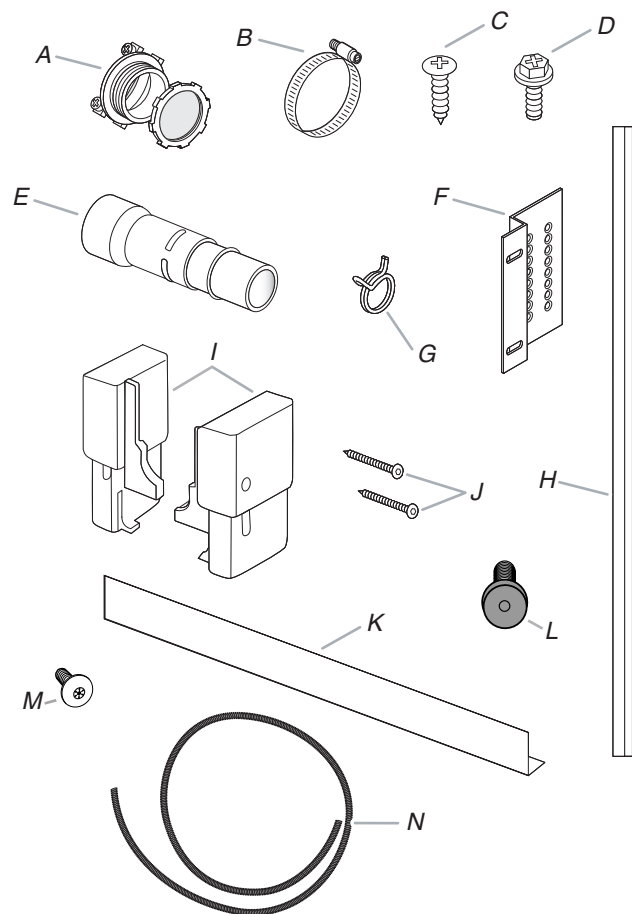
A. \frac{3}{4} " UL Listed/CSA Approved strain relief B. 1.25" hose clamp C. Mounting bracket screws (8) D. Unit mounting screws (4) E. Drain hose connector F. Mounting brackets (4) G. Drain connector spring clamps (2) H. Trim strips (2) I. Toe kick brackets (2) J. Toe kick bracket screws (2) K. Toe kick trim L. Panel fasteners (on some models) (2) M. TORX † screws (on some models) (10) N. Drain hose
