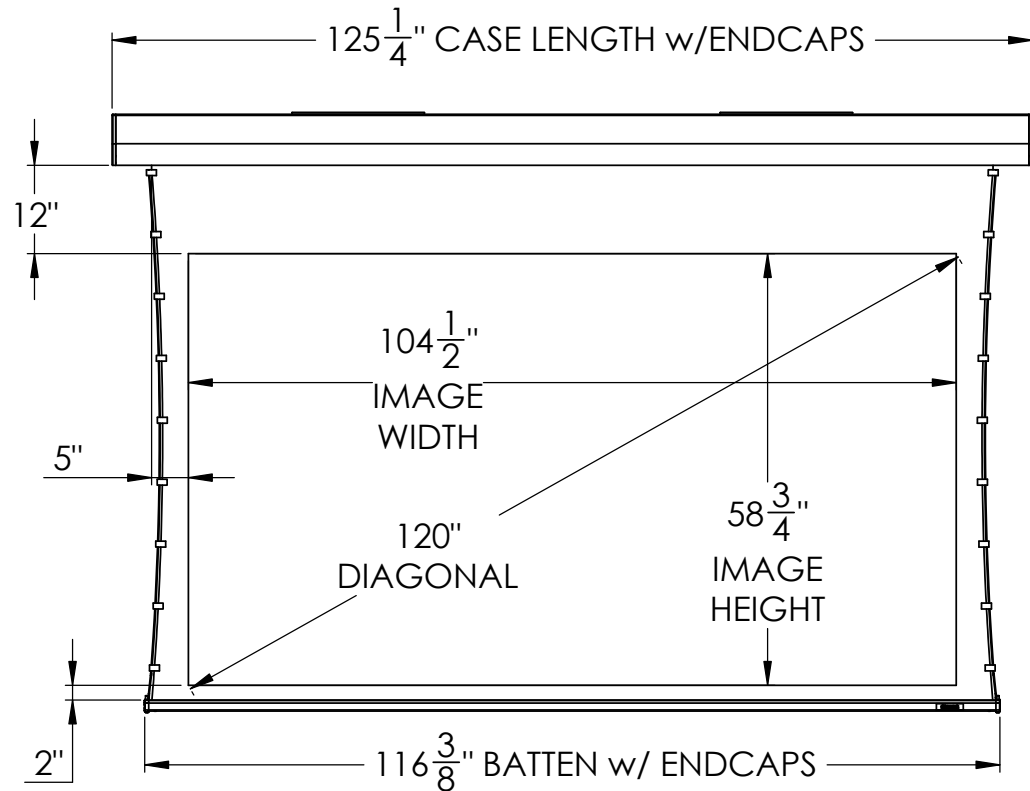
FRONT VIEW
