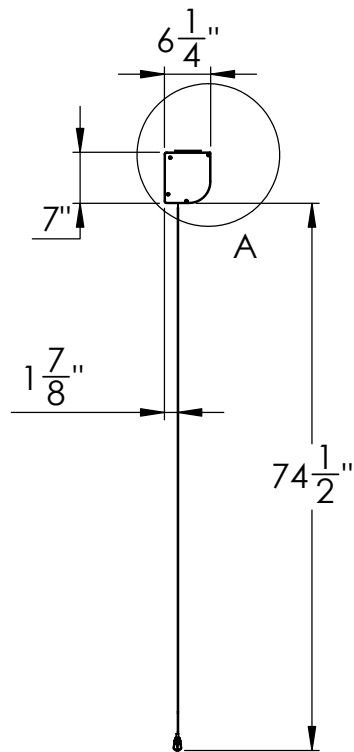
SIDE VIEW
