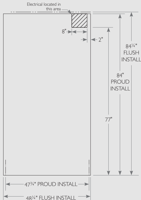
FRONT VIEW FIGURE 2 - ROUGH OPENING
