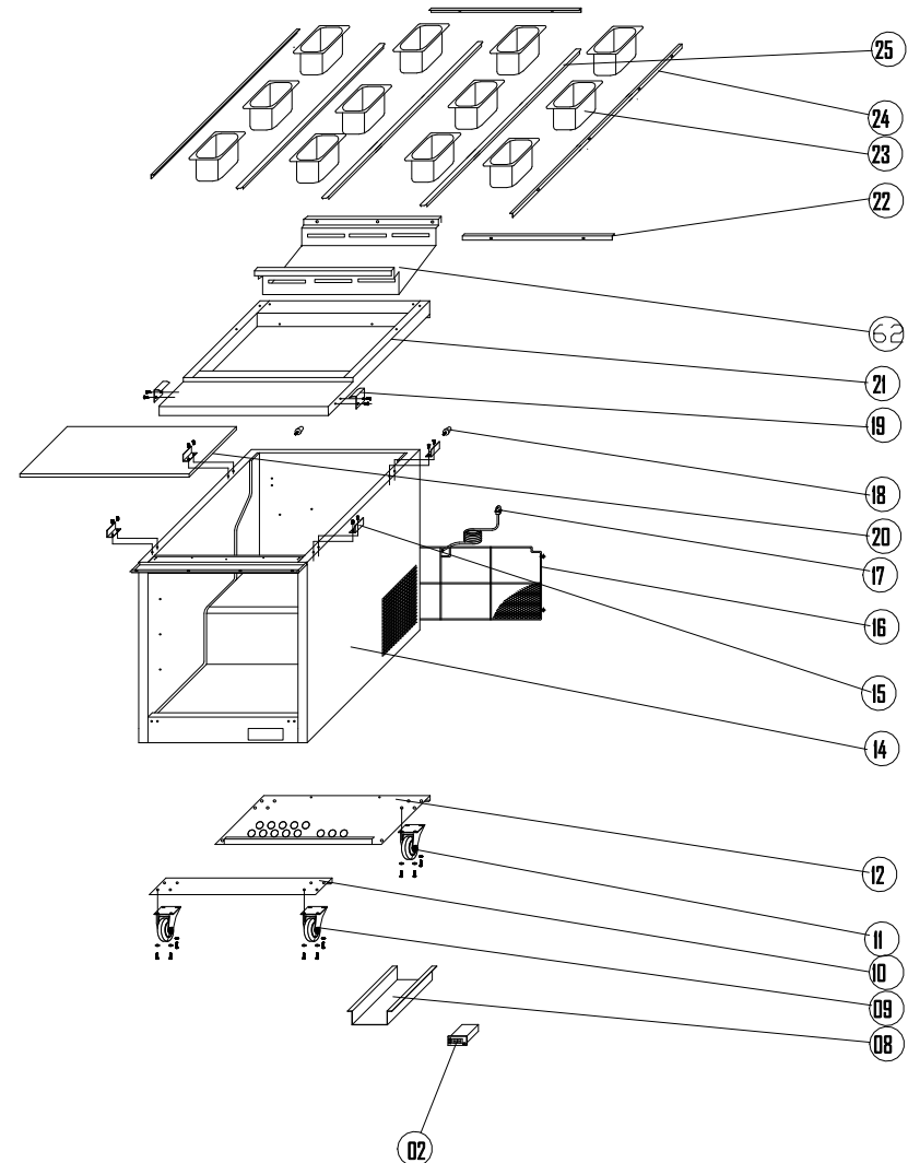
EXPLODE OF KCHMT29.12.2D
