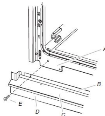
A. Oven frame B. Vent tab C. Oven vent D. Bottom vent trim E. #8-18 x \frac{3}{8} " (9.5 mm) screw
