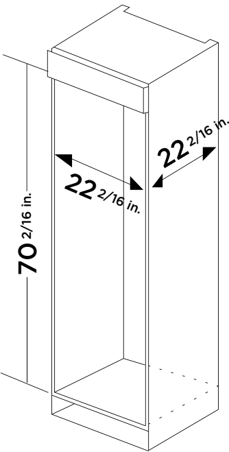
CUT-OUT DIMENSIONS
