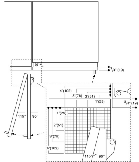
Door opening angle
