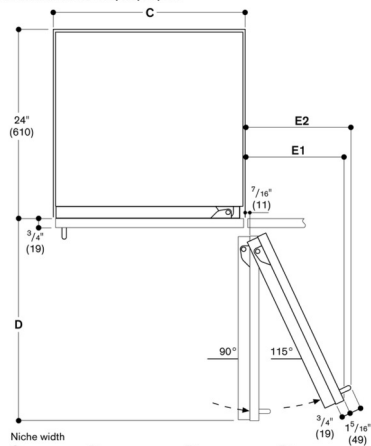
Wall clearance RB 472/RC/RF/RW
