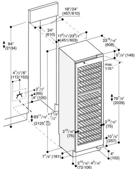
Wall clearance RB 472/RC/RF/RW
