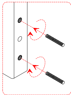
Detail 'A'
