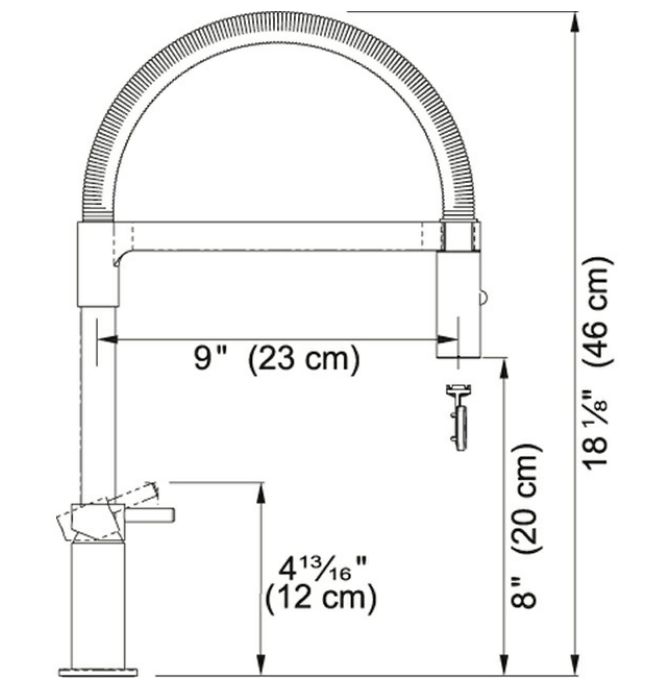
Technical Drawing
