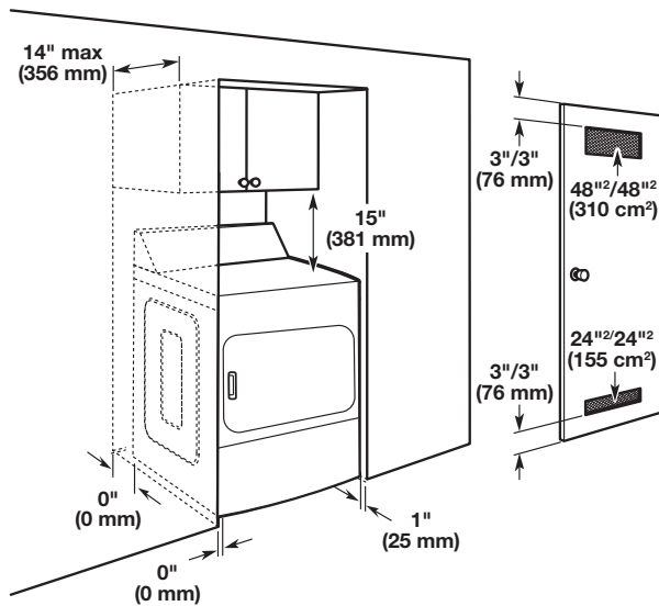
Closet Installation
