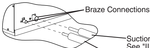
Rack System-Braze Connection
