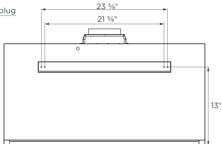
REAR
