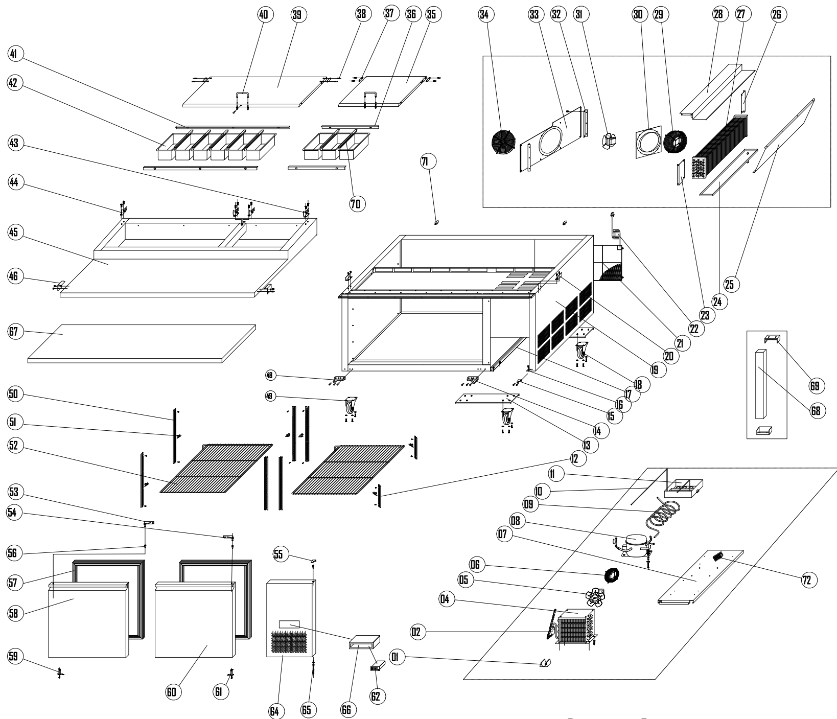
EXPLODE OF KCHPT72.9
