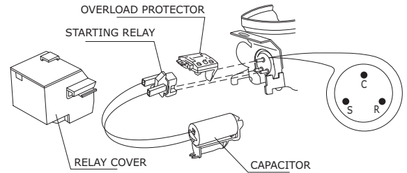
Electrical Relay and Overload Protector
