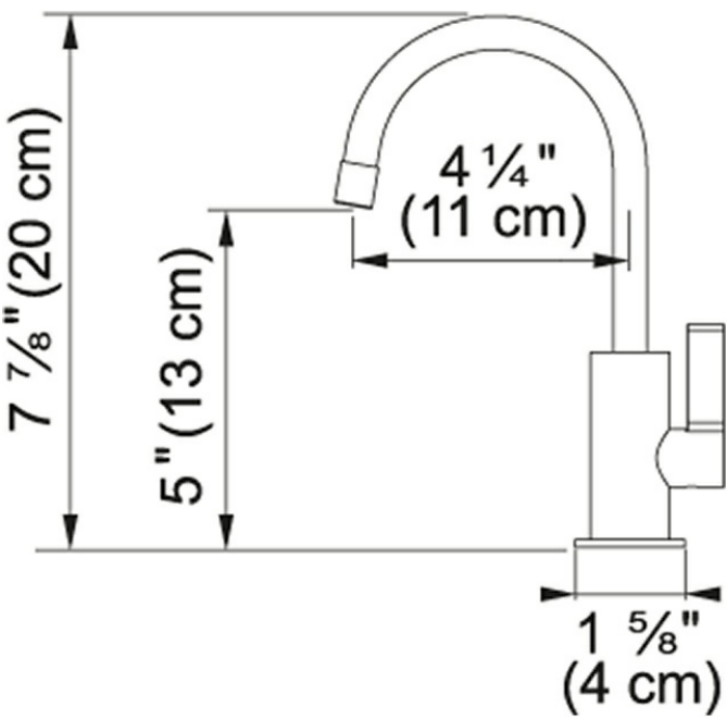
Technical Drawing
