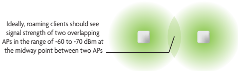
XAP-1410 Multiple AP Coverage and Overlap
