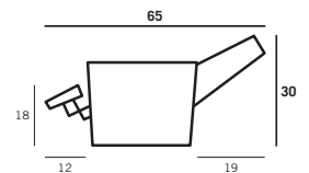
Side View (standard mechanism, fully reclined)
