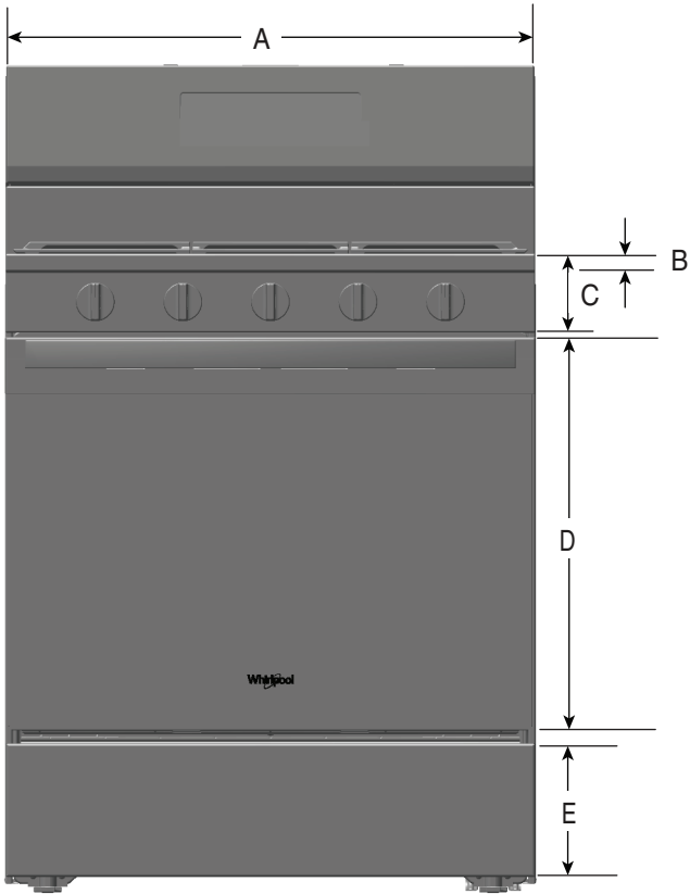
VISTA FRONTAL
