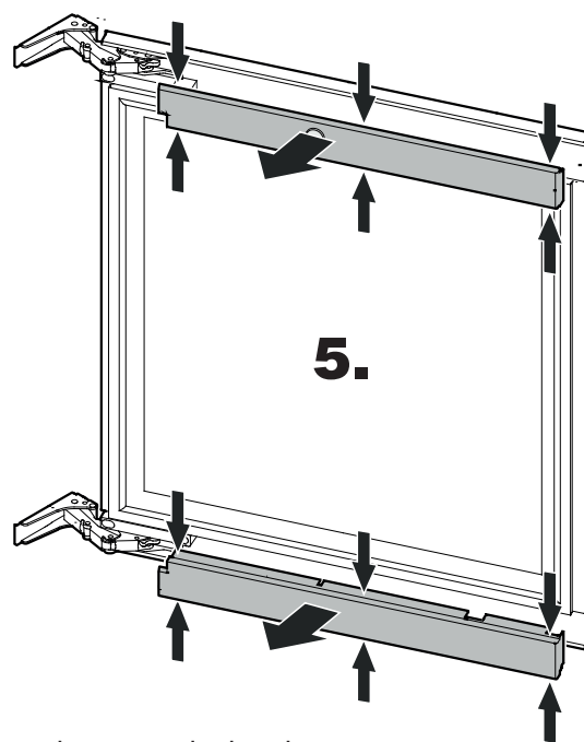
5. Compress the covers in the places shown, release and remove.
