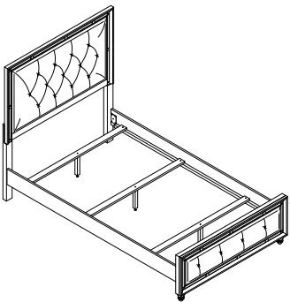
COMPLETED FULL BED ASSEMBLY
