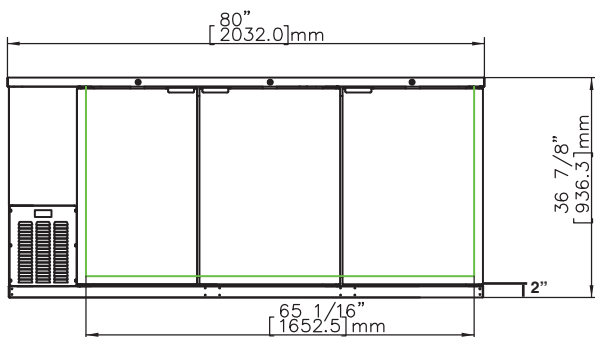
BB80-G(-S) Front View
