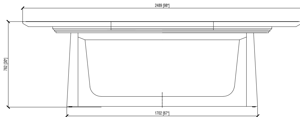
FRONT VIEW (CLOSE)
