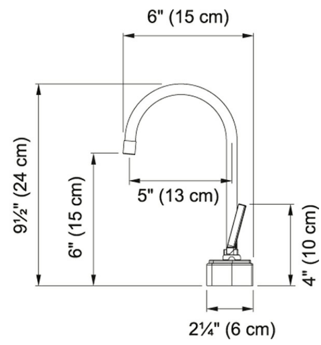
Technical Drawing
