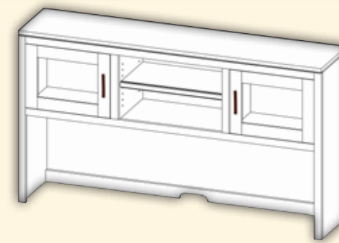
Hutch Top #88551 . . . For 54" Credenza 14Dx52Wx36H #88552 . . . For 60" Credenza/Desk 14Dx58Wx36H #88553 . . . For 66" Credenza/Desk 14Dx64Wx36H #88554 . . . For 72" Credenza/Desk 14Dx70Wx36H
