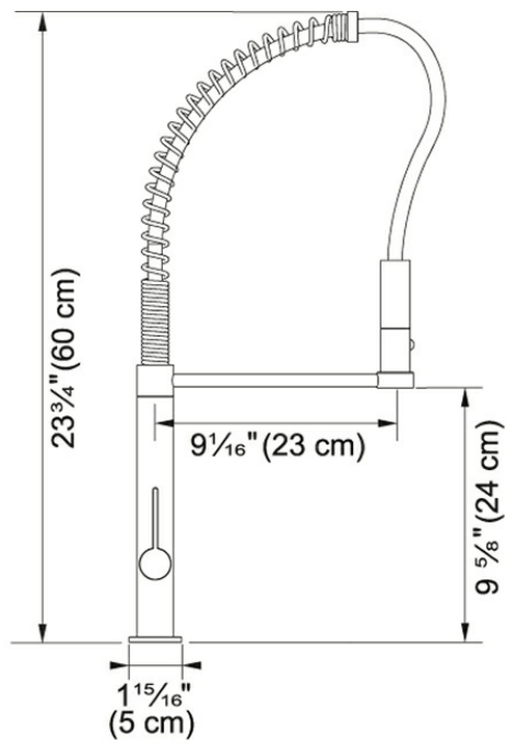
Technical Drawing
