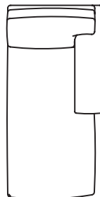
11518-LAF Library Left Arm Facing Sofa Overall: H35½ W82 D40 Seat: W72 D23 Seat: H20 Arm:H22½
