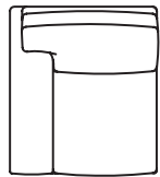
11516-LAF Library Left Arm Facing Chair Overall: H35½ W34 D40 Seat: W24 D23 Seat: H20 Arm:H22½
