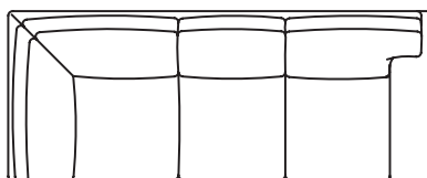
11519-RAF Library Right Arm Facing Sofa with Built-In Corner Overall: H35½ W98 D40 Seat: W71 D23 Seat: H20 Arm:H22½
