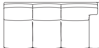
11518-RAF Library Right Arm Facing Sofa Overall: H35½ W82 D40 Seat: W72 D23 Seat: H20 Arm:H22½
