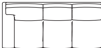
11518-LAF Library Left Arm Facing Sofa Overall: H35½ W82 D40 Seat: W72 D23 Seat: H20 Arm:H22½
