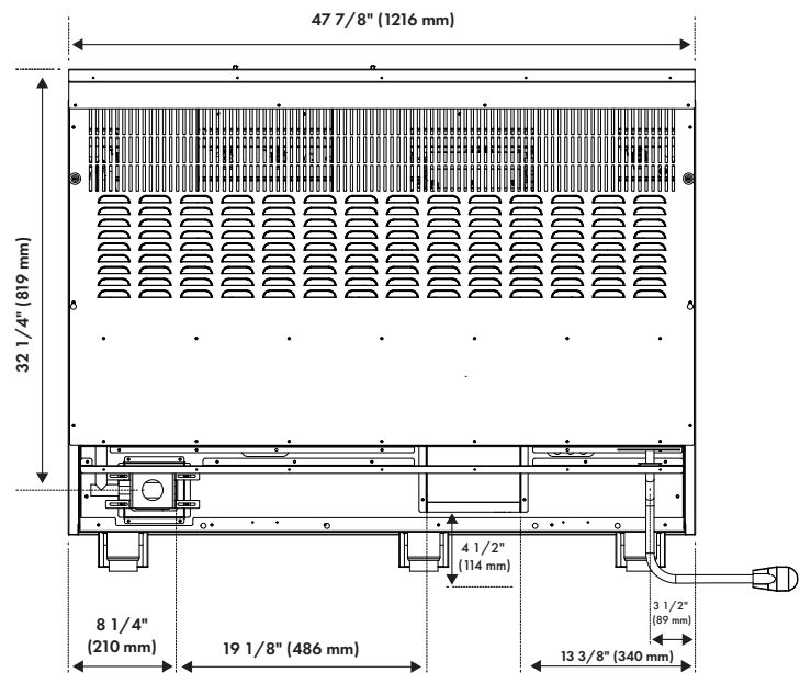
BACK VIEW
