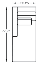
LTD5201-81 LAF Chaise W 33.25 D 77.25 H 37.5
