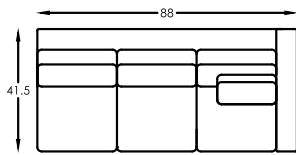
LTD5201-52 RAF Sofa W 88 D 41.5 H 37.5
