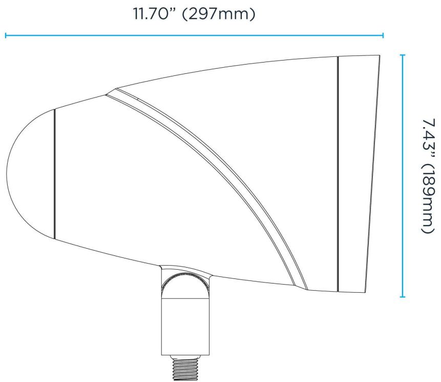
SLS LS6T Speaker Side View
