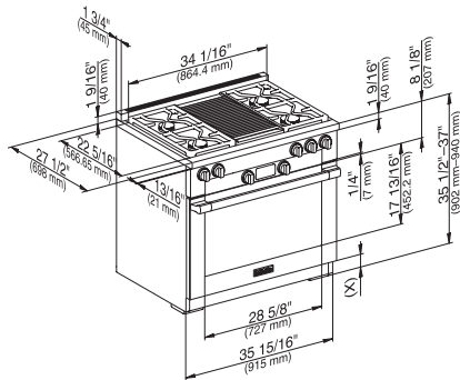
HR1135G, HR1135-1 (installation drawing)
