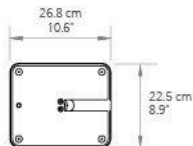
Bottom Plate
