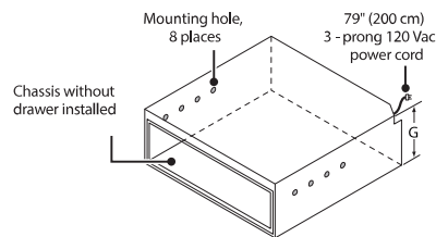
CHASSIS DIMENSIONS
