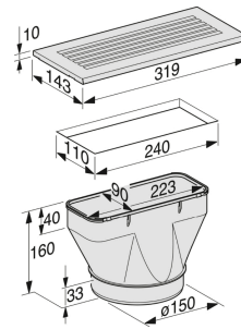
DUU151 (installation drawing)
