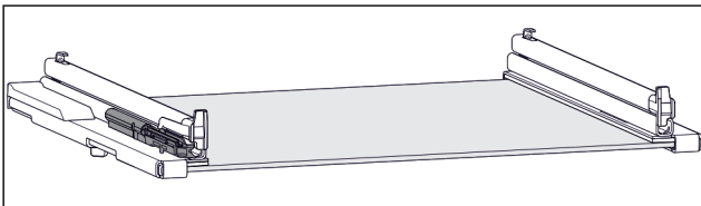
Fig. 106 Damping mechanism
