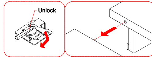
Detail 'E'
